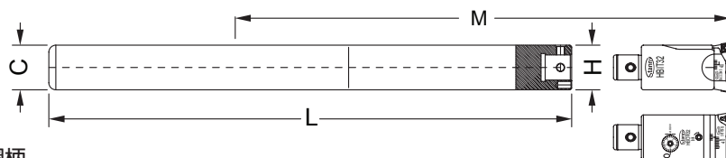
鎢鋼柄 Carbide Shank
