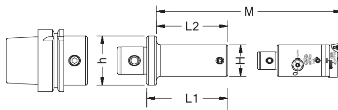
縮徑接桿 Stepped Spacer
