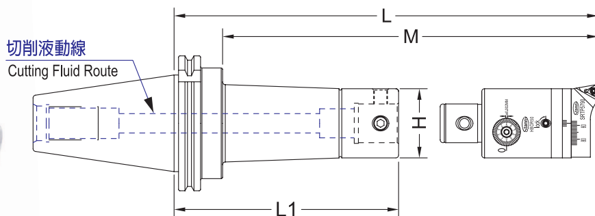
DIN69871A 搪孔刀柄 DIN69871A Taper Shank
