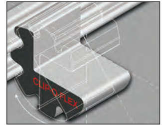
The flexible clip-in profile permits hanging-on and out at angles of 0/40/80° or 0/45/90° that can be changed at any time, and can be moved to the side.
