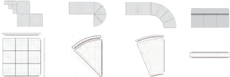
Quadratic 910 x 910 mm 45° Inner angle 910 mm x 45° 22,5° Outer angle 910 mm x 22.5° Safety marking 910 x 100 mm
